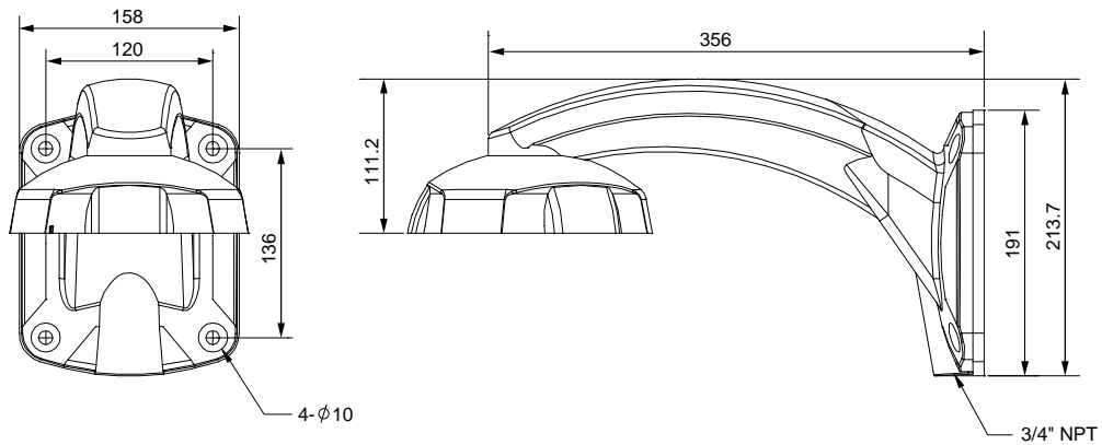
● Wall Mount Bracket
